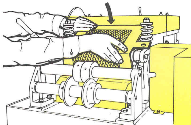
ROLL FEEDER
